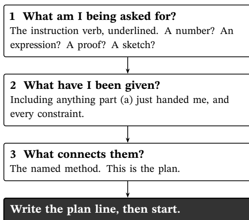
Figure 9.1: The thirty-second opening. Three questions, then the plan line, then the mathematics.
