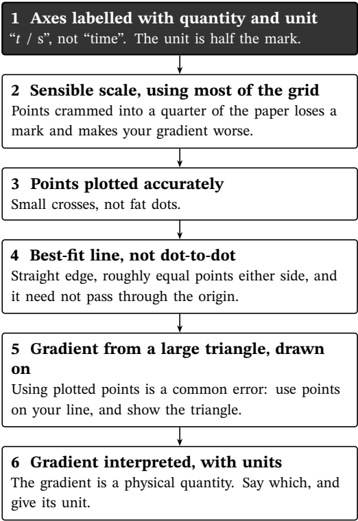
Figure 17.1: The six graph marks. They are the same on nearly every paper, and five of them require no physics at all.
