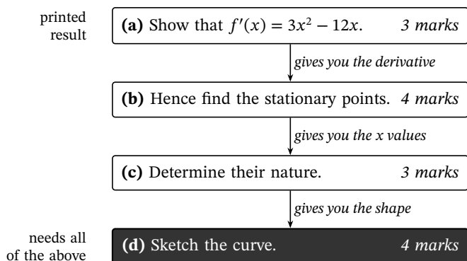
Figure 18.1: The ladder. Each part hands the next one its input, and the printed result in a “show that” is yours to use even if you couldn’t derive it.
