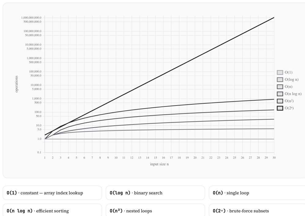
Big-O complexity comparison chart on logarithmic scale
