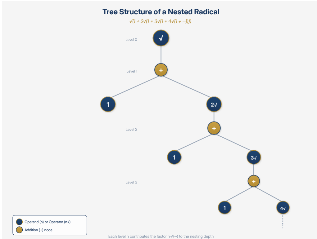
Figure 1: Tree structure of a nested radical expression, illustrating how each level of nesting branches into its constituent terms.
