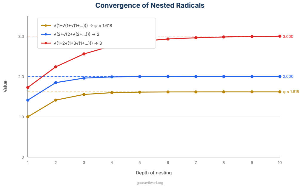
Figure 3: Convergence of partial nested radicals toward their limits: the golden ratio \varphi , the integer 2, and Ramanujan's identity for 3
