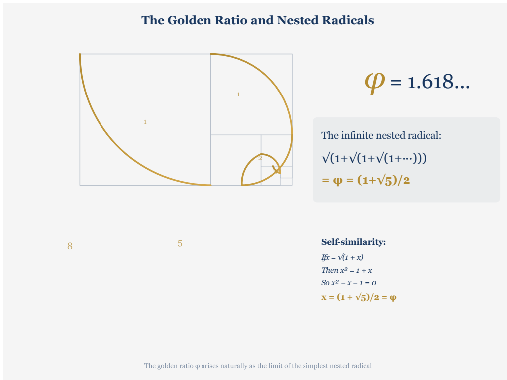
Figure 2: The golden spiral arising from the constant nested radical \sqrt{1 + \sqrt{1 + \sqrt{1 + \cdots}}} = \phi , illustrating the geometric connection between nested radicals and the golden ratio.
