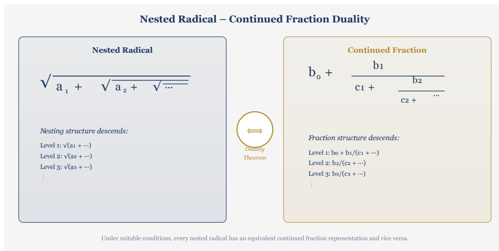
Figure 5: The duality between nested radicals and continued fractions: both representations converge to the same algebraic quantity via different recursive structures.
